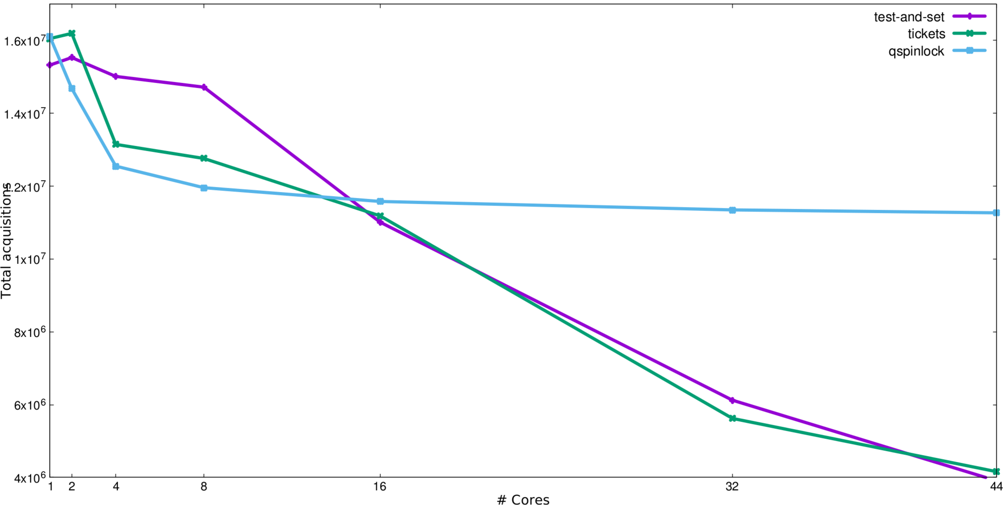
Total lock acquisitions as number of cores increases (10s total, 500ns critical section)
